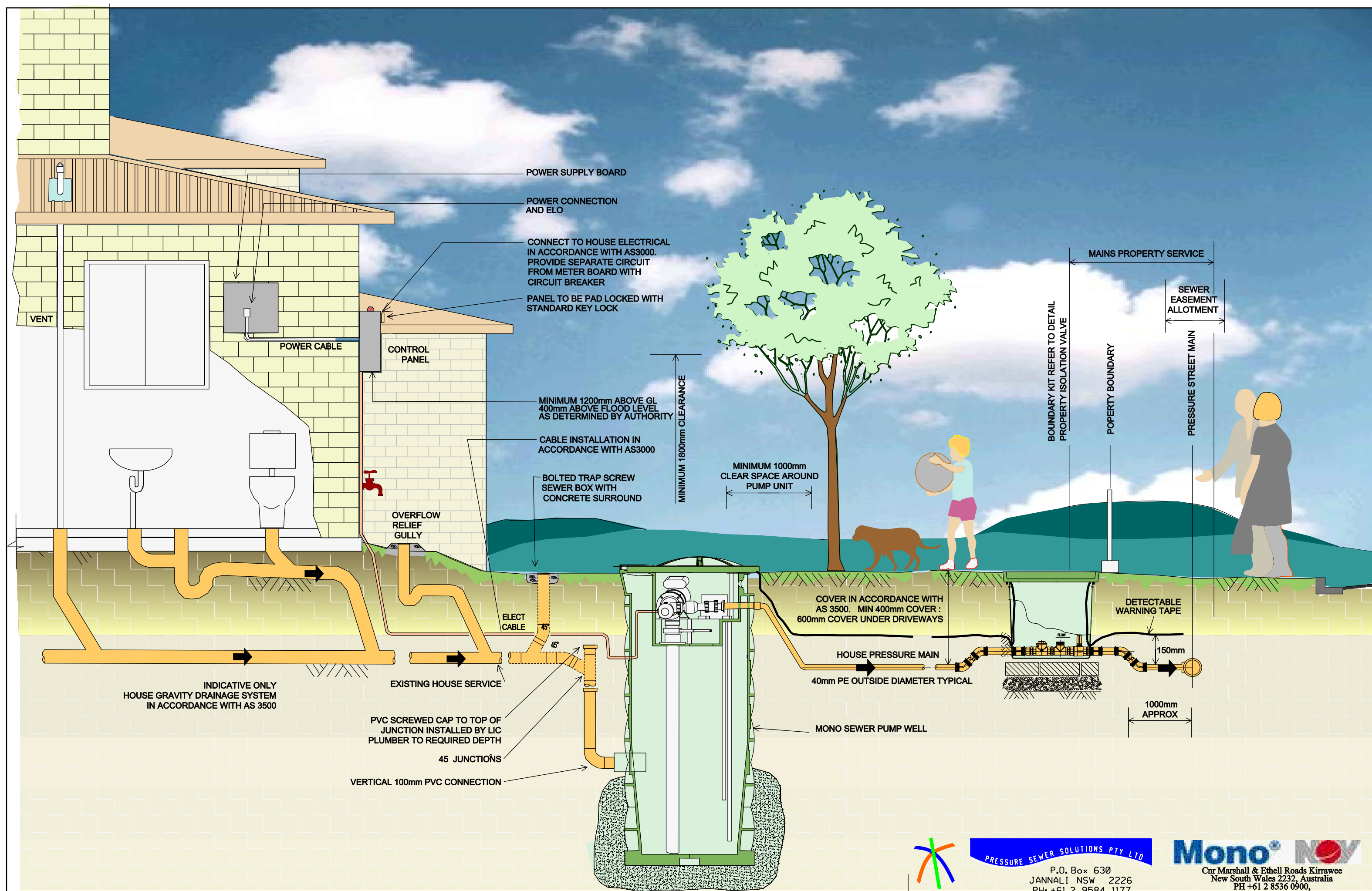
TYPICAL HOUSE CONNECTION DETAIL
