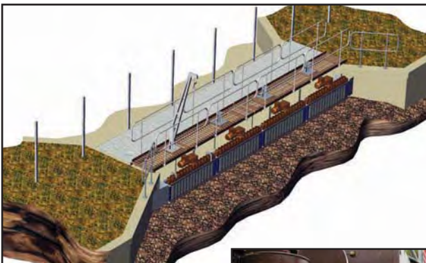
4 Discreens installed at a lagoon intake to screen abstracted water
