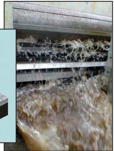
The Mono Stormscreen an economical solution to storm overflow applications
