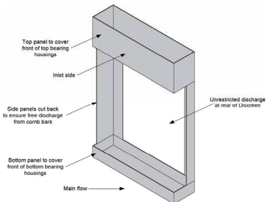
Figure 7 Support frame
