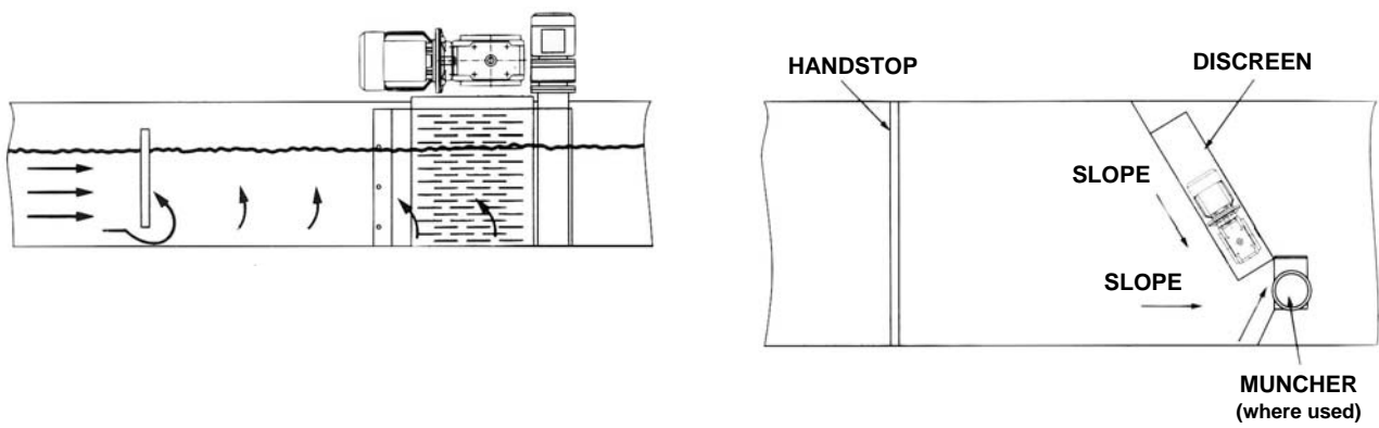
Figure 3 Hand Stop
