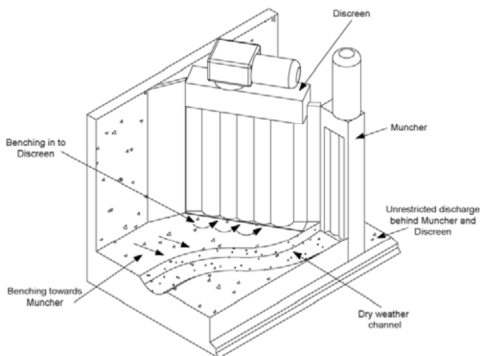
Figure 6 Recommended channel design
