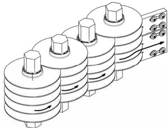
Figure 1 Operating Principle
