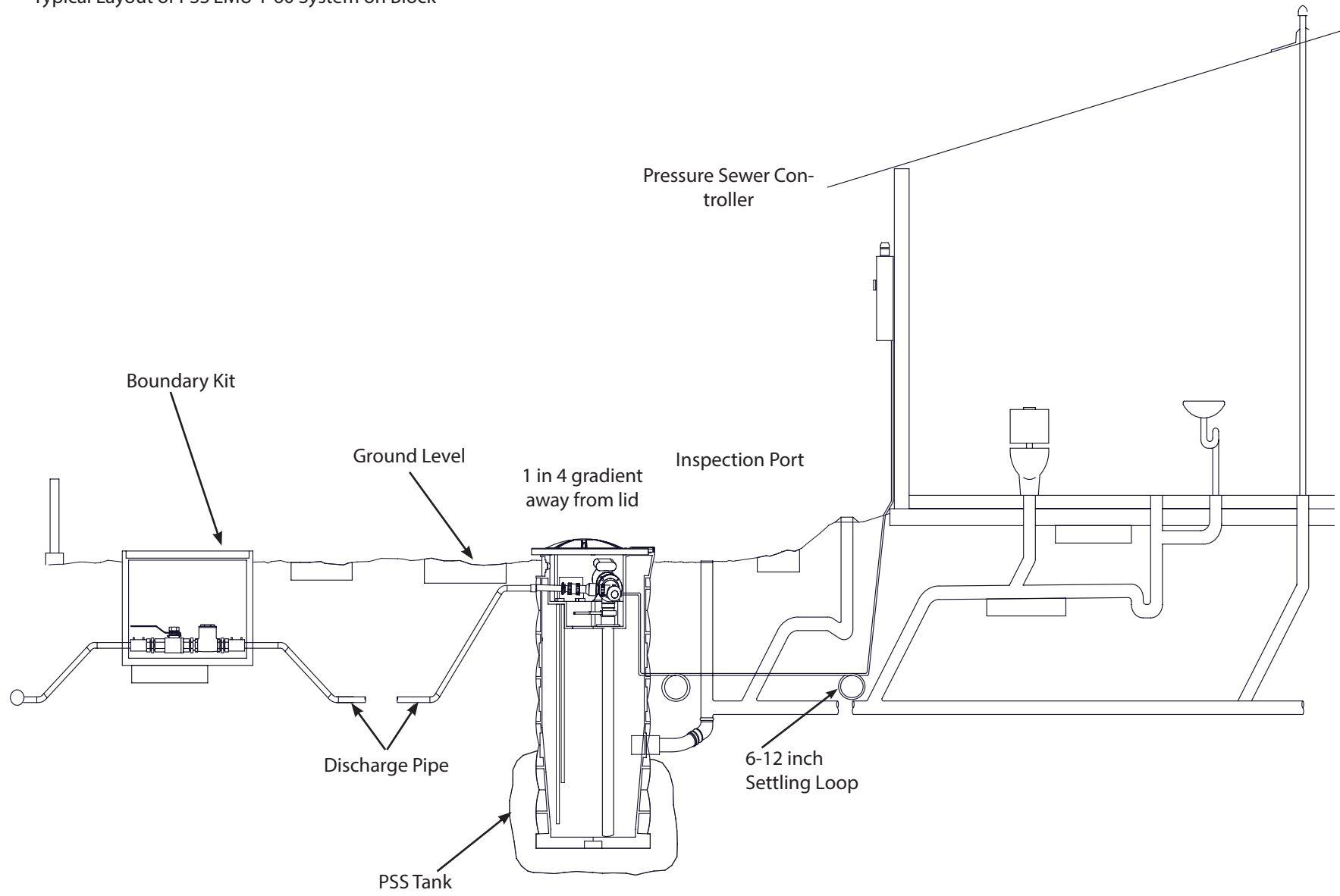
Typical Layout of PSS EMU 1-60 System on Block
